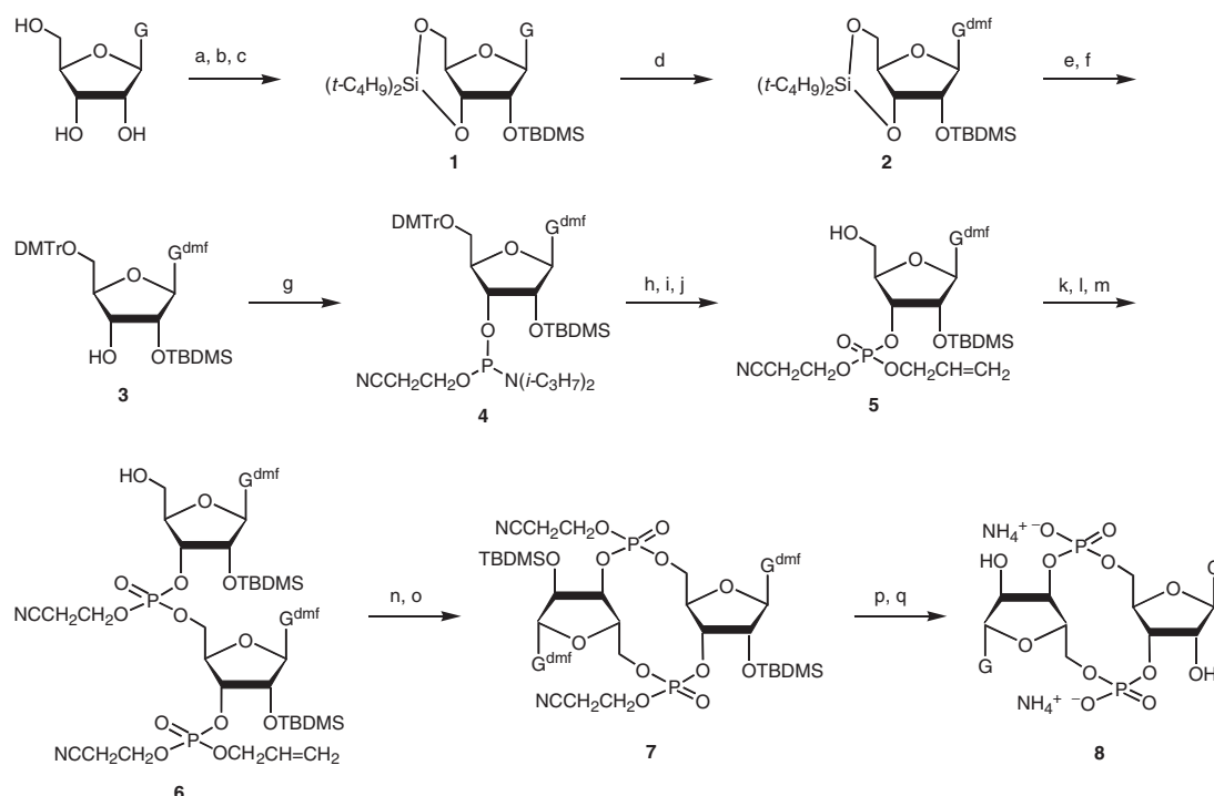
Scheme 1. (a) (t\text{-C}_4\text{H}_9)_2\text{Si}(\text{OTf})_2 , 0 °C, 45 min; (b) imidazole, 25 °C, 30 min; (c) TBDMSCl, 60 °C, 2 h; (d) (\text{CH}_3)_2\text{NCH}(\text{OCH}_3)_2 , 50 °C, 5 h; (e) HF·pyridine, pyridine, \text{CH}_2\text{Cl}_2 , 0 °C, 2 h; (f) DMTrCl, pyridine, 25 °C, 12 h; (g) \text{NCCH}_2\text{CH}_2\text{OP}[\text{N}(\text{i-C}_3\text{H}_7)_2]\text{Cl} , 2,4,6-collidine, N -methylimidazole, THF, 25 °C, 1 h; (h) allyl alcohol, IMP, MS 3A, \text{CH}_3\text{CN} , 25 °C, 30 min; (i) a 6.7% BPO/toluene solution, 25 °C, 5 min; (j) a 20% \text{Cl}_2\text{CHCOOH}/\text{CH}_2\text{Cl}_2 solution, 25 °C, 10 min; (k) the phosphoroamidite 4 , IMP, MS 3A, \text{CH}_3\text{CN} , 25 °C, 30 min; (l) a 6.7% BPO/toluene solution, 25 °C, 5 min; (m) a 20% \text{Cl}_2\text{CHCOOH}/\text{CH}_2\text{Cl}_2 solution, 25 °C, 10 min; (n) NaI, acetone, reflux, 2 h; (o) TPSCl, N -methylimidazole, 25 °C, 36 h; (p) conc. aq. \text{NH}_3\text{--CH}_3\text{OH} (1:1 v/v), 50 °C, 12 h; (q) (\text{C}_2\text{H}_5)_3\text{N}\cdot 3\text{HF} , 25 °C, 12 h.
